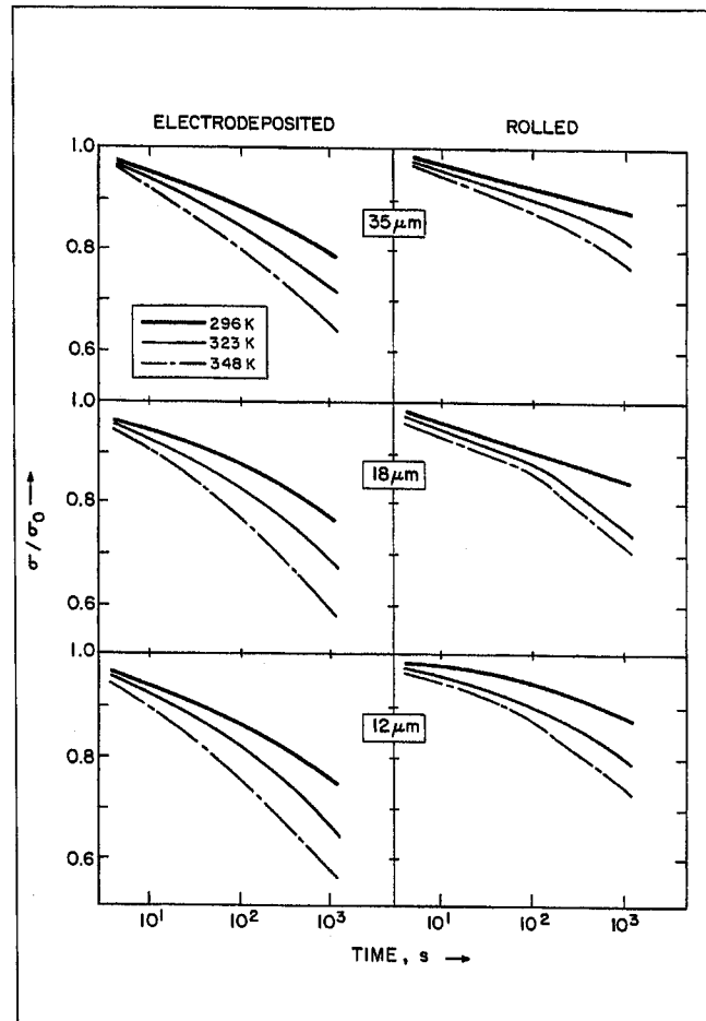
Fig. 2. Stress relaxation curves for 12, 18, and 35 \mu\text{m} thick electrodeposited and rolled foils ( \sigma_0 near \sigma_y ; for \sigma_y values, see Fig. 8).
