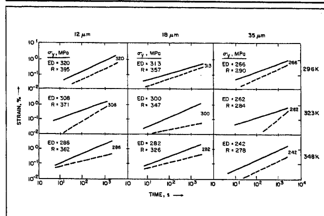
Fig. 8. A comparison of creep for ED (—) and R (---) foils at and near yield stress.
