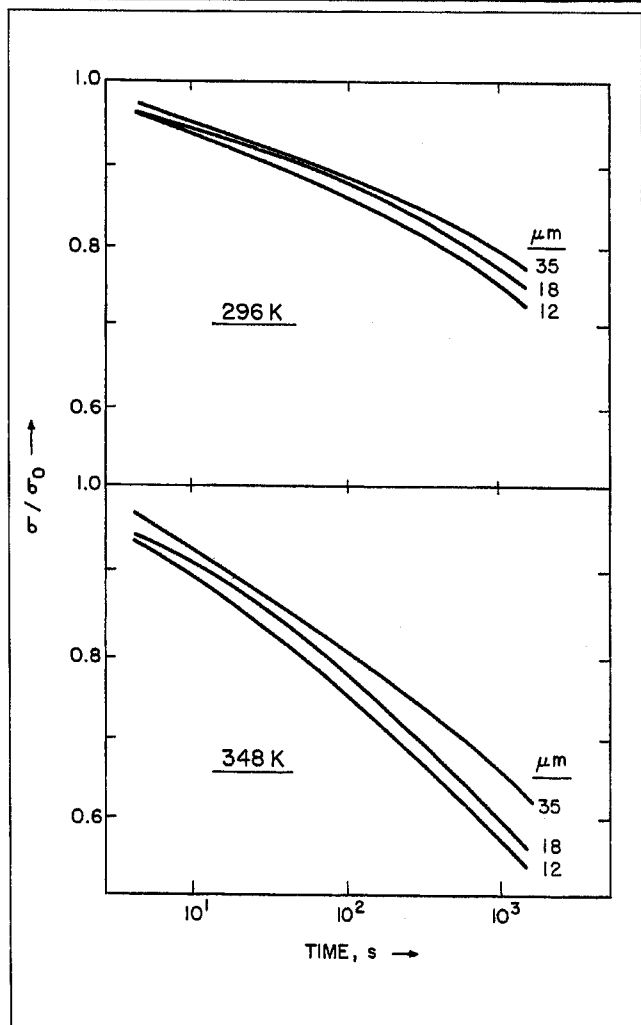
Fig. 3. Effect of thickness of electrodeposited foil on stress relaxation.
